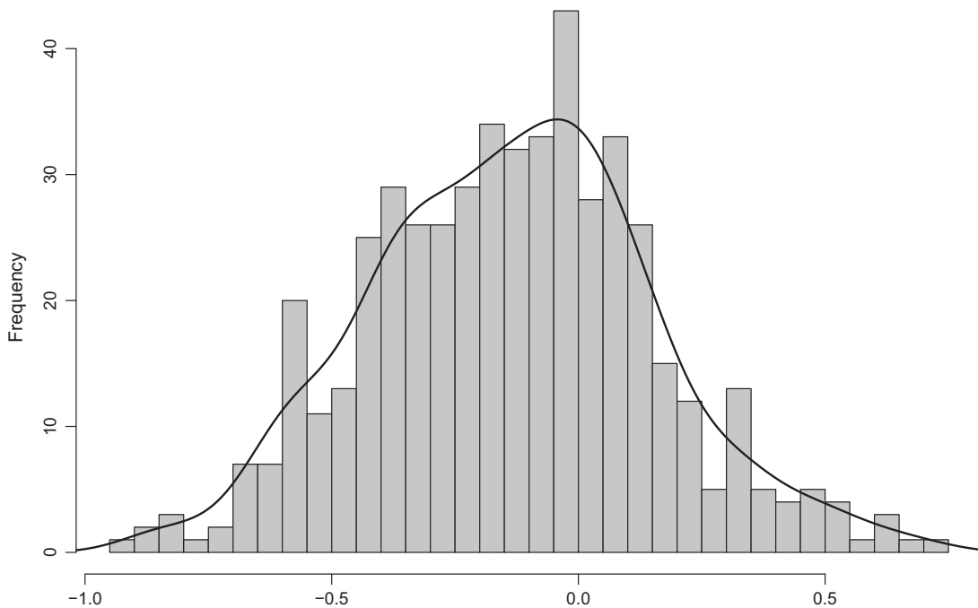
Fig. 1. Beta(1, 3.7) – Beta(1.3, 2.3). We generate 1000 samples of 500 data points which are randomly drawn from the Beta(1, 3.7) – Beta(1.3, 2.3). The figure shows that the Beta(1, 3.7) – Beta(1.3, 2.3) distribution appears to be asymmetric with a slightly longer left tail. We calculate skewness, denoted by Skew, and the asymmetry measure for each of the 1000 samples of 500 data points. This gives us a total of 1000 values of Skew and Asym for each of the three distributions. Finally, we calculate the sample means, standard errors and t-statistics for both Skew and Asym. The statistics are reported in Table 1.
